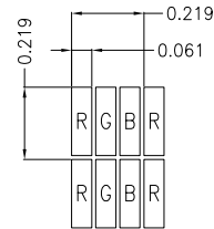
PIXEL DETAIL (SCALE 40:1)
